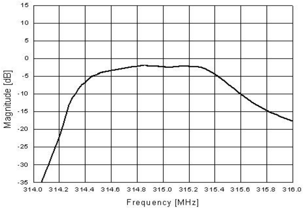
Frequency Response
